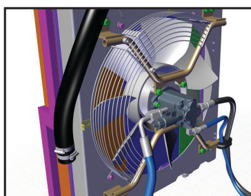
Hydraulic Fan Drive for Radiator
